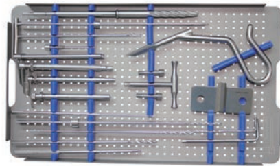
111410100 Universal Tibial Nail II Instrument Case
